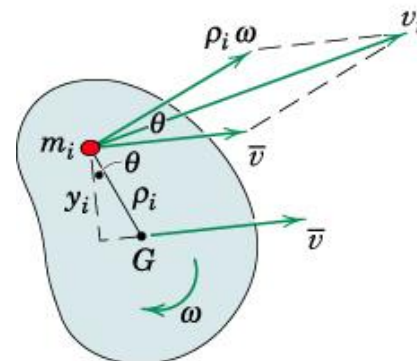
(c) General Plane Motion
